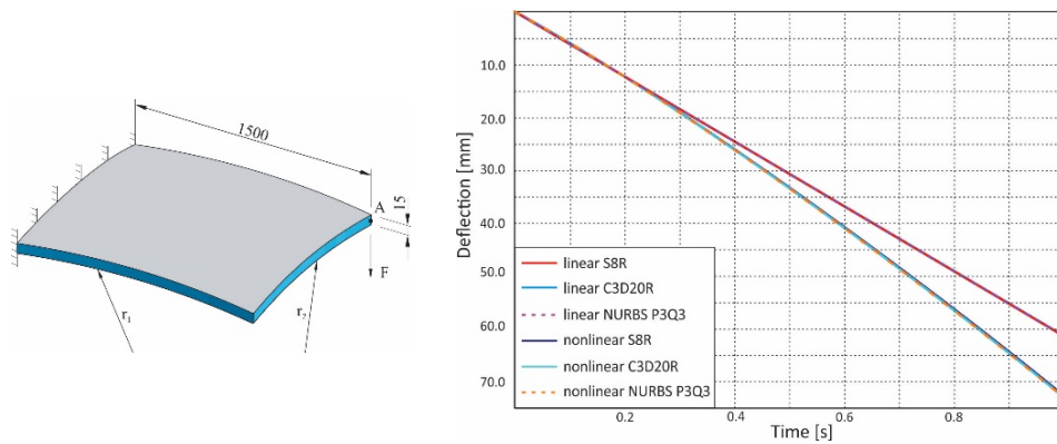
Fig. 5 a) Double-curved shell exposed to single force; b) linear (straight line) and nonlinear (curved line) deflection of point A
