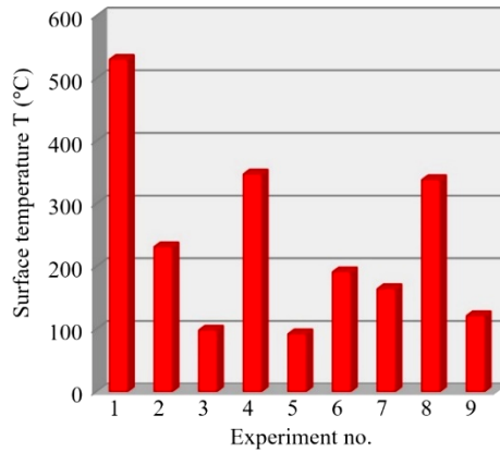
Fig. 4 Workpiece surface temperature values
