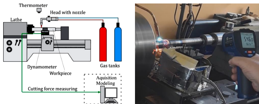
Fig. 2 Experimental setup
