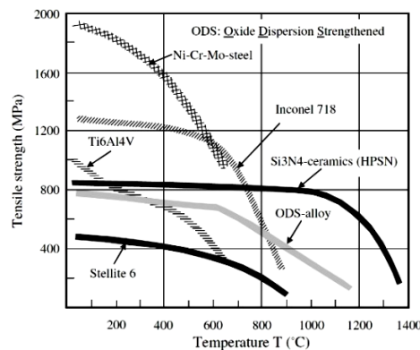
Fig. 1 Tensile strength reduction due to temperature
