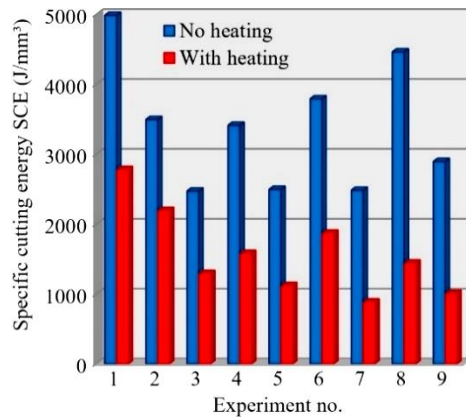
Fig. 3 Specific cutting energy values
