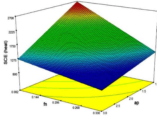
Fig. 5 Specific cutting energy model response
